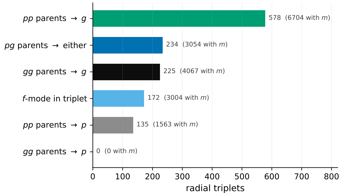
(b) direct: two parents \rightarrow one daughter 1344 radial triplets
