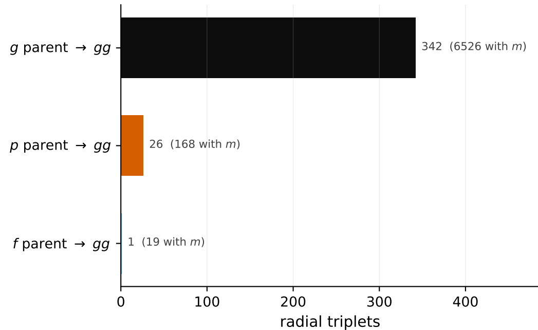
(a) parametric: one parent \rightarrow two daughters 369 radial triplets
